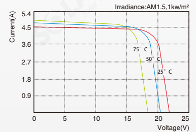
SLP080S-12M I-V Curves
